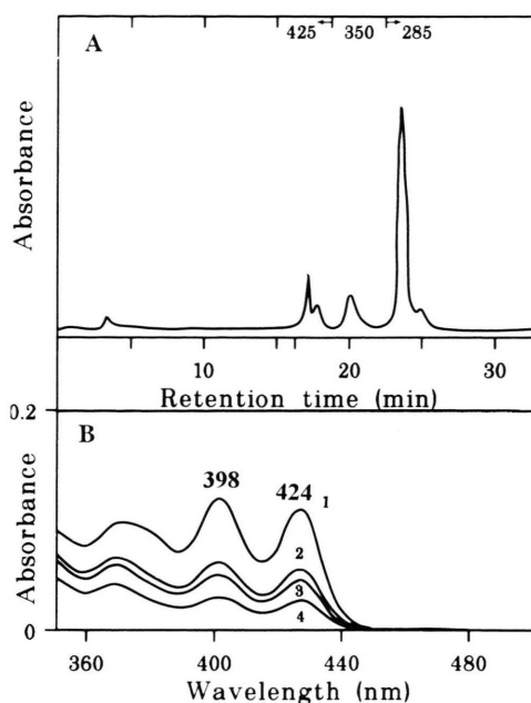
Fig. 1. HPLC separation (A) and optical absorption spectra (B) of carotenoid extracts from cell-free phytoene desaturase assays. To (A): (a) \zeta -carotene, (b) phytofluene, (c) phytoene. To (B): 1 = control, 2 = addition of 2 \mu\text{M} , 3 = addition of 6 \mu\text{M} , 4 = addition of 10 \mu\text{M} of WL110547 to the assay. Two maxima for \zeta -carotene absorption are noted at spectrum 1.
